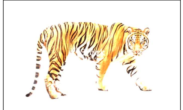
Identity Kernel
