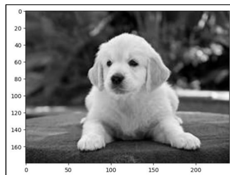
Grayscale
